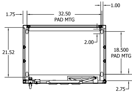
SECTION C-C
